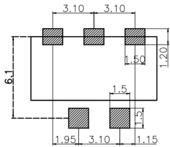
PCB Layout
